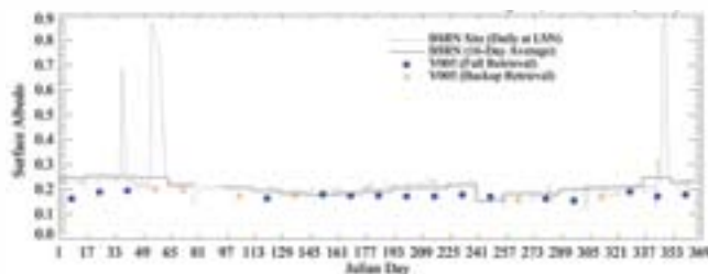
Comparison of the MODIS 500-m albedo product with field measurements at the ARM/SGP Central Facility #C01 (2003)
