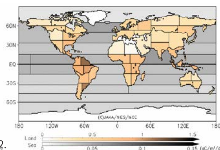
Figure 21. L4A global CO 2 flux. A sample map of regional CO 2 flux estimates, August 2012.
