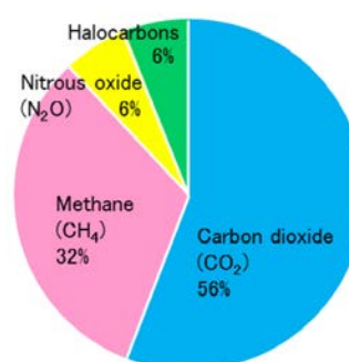
Figure 4. Contributions of primary greenhouse gases to the increase in atmospheric temperatures. The above figures are based on the best estimates of radiative forcing from 1750 to 2011. (Source: IPCC Fifth Assessment Report)
