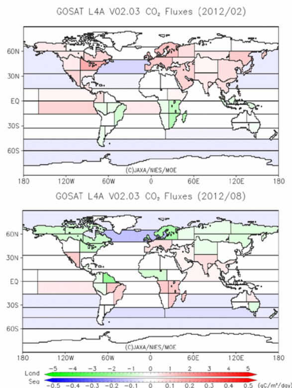
Figure 5. Sample estimates of global \text{CO}_2 sources and sinks ( \text{gC/m}^2/\text{day} ). February (upper), August (lower), 2012.
