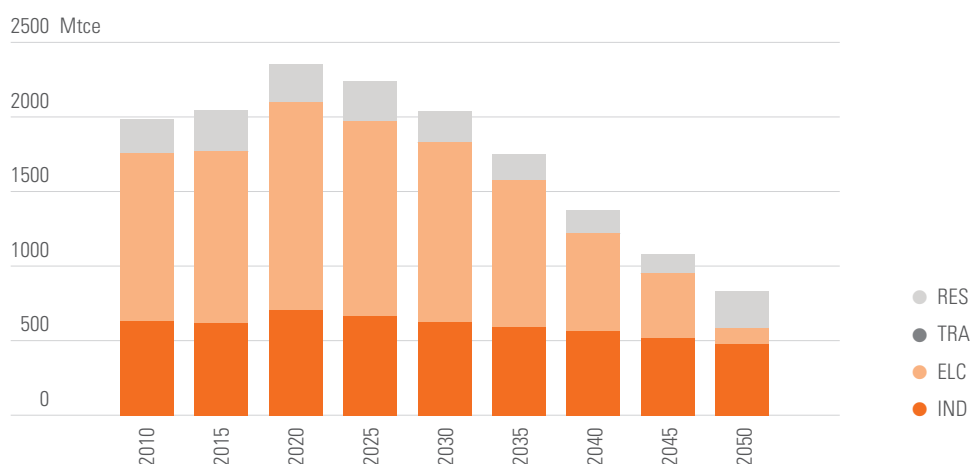
Figure 7. Coal consumption by sector under PEAK-2025 scenario
