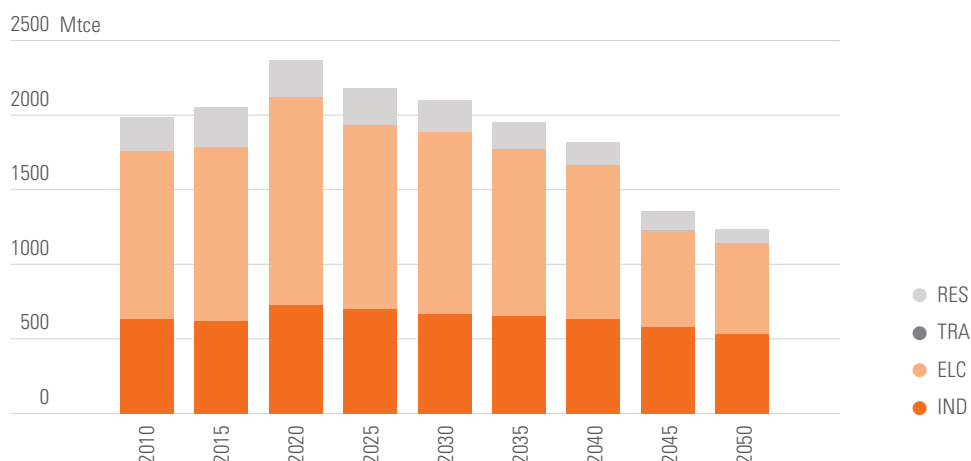
Figure 2. Coal consumption by sector under PEAK-2030 scenario
