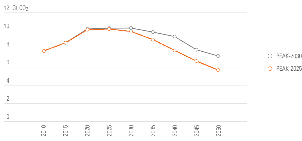
Figure 6. CO 2 emissions under 2025 vs 2030 peaking scenarios
