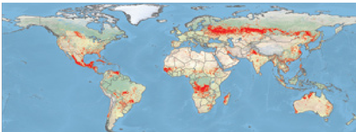
Global distribution of MODIS active fire detections for May 2006 from the FIRMS system
