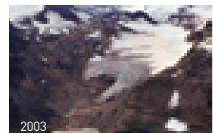
Retreat of South Cascade Glacier, USA. Photographs from the US Forest Service (1928) and the US Geological Survey (1966, 1979, 2003)
