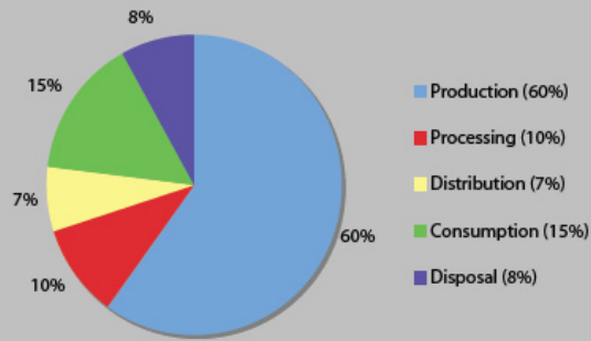
Estimated Percentage of Greenhouse Gas Contributions from U.S. Food System by Sector
