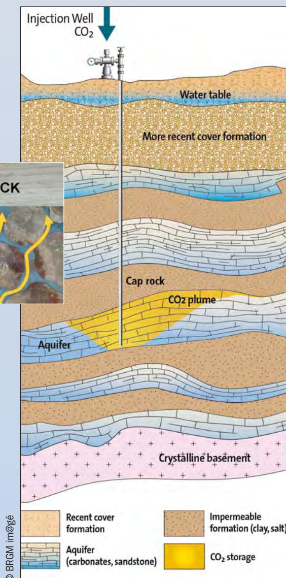
Figure 1 The injected CO 2 , which is lighter than water, tends to rise and is stopped by overlying impermeable rocks.
