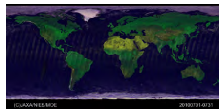
Figure 19. CAI Level 3 global reflectance distribution synthesized from cloud-free data obtained between July 1 and 31, 2010.
