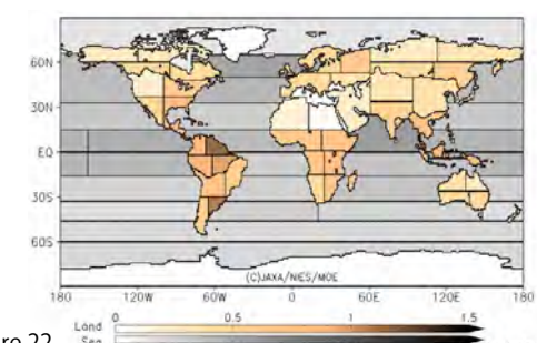
Figure 22. L4A global CO 2 flux. A sample map of regional CO 2 flux uncertainties, August 2012.
