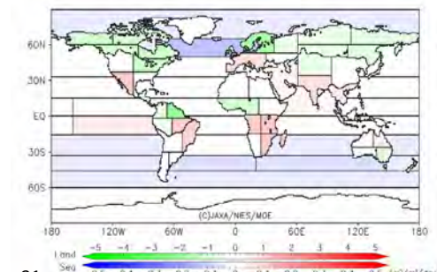
Figure 21. L4A global CO 2 flux. A sample map of regional CO 2 flux estimates, August 2012.
